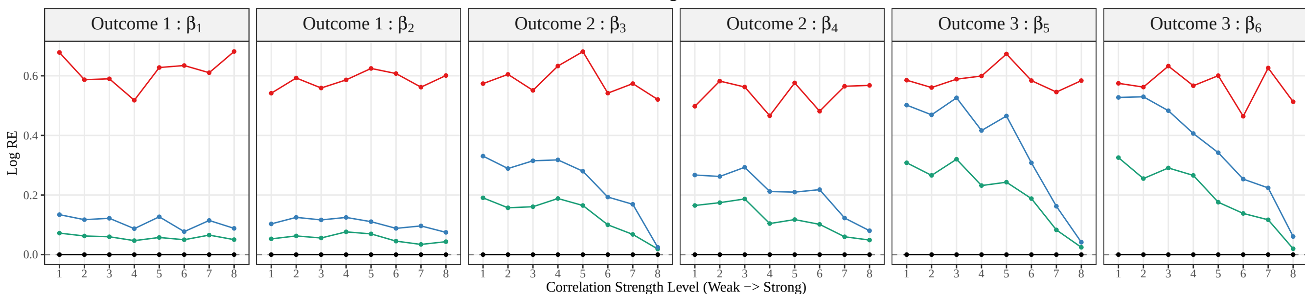
Variance: Bias
